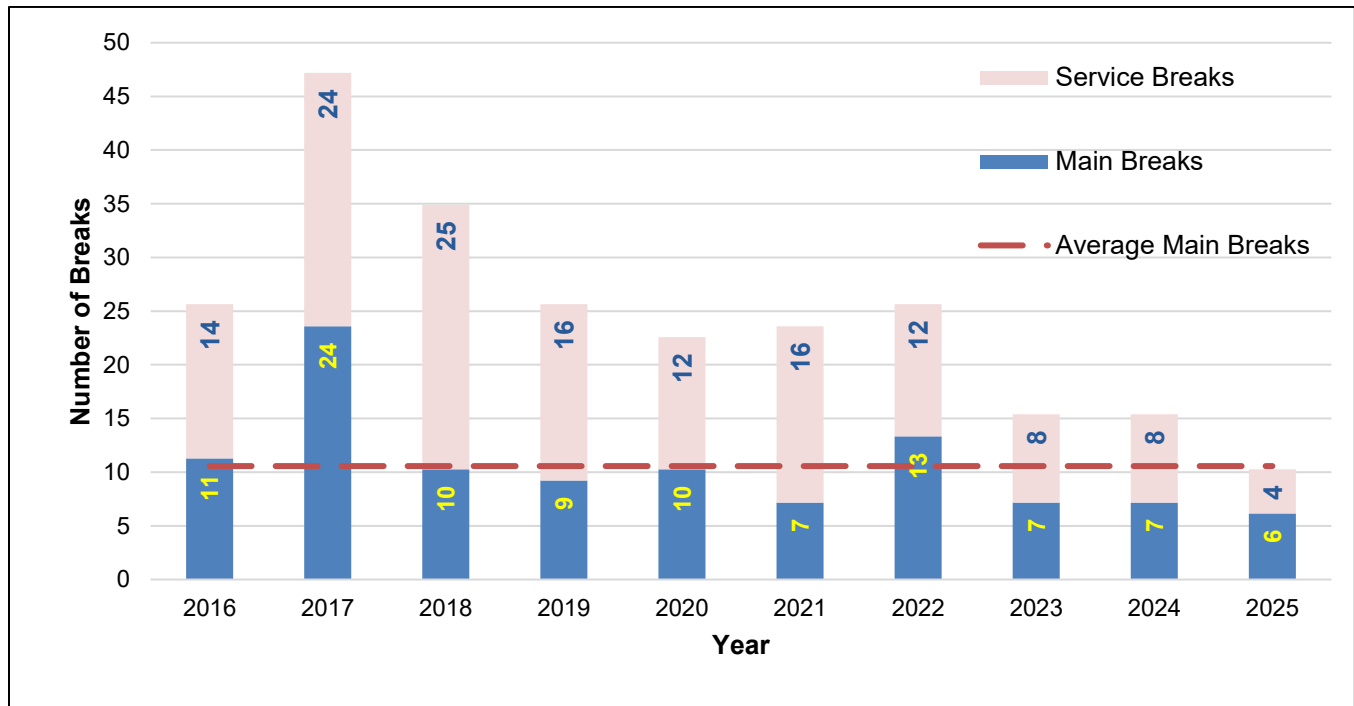
FIGURE 3 - WATERMAIN/SERVICE BREAK HISTORY
