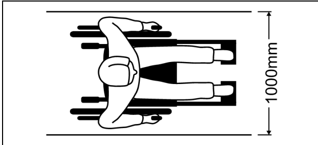
3.8.3.2.(1) Clear Width
